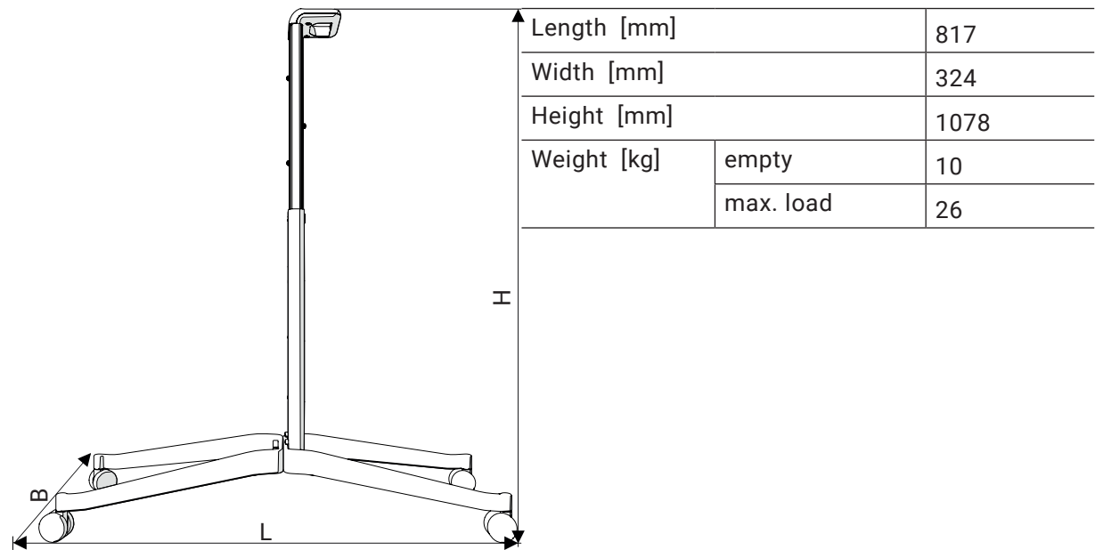
Fig. 2 Dimensions of the "Meeting" office caddy
