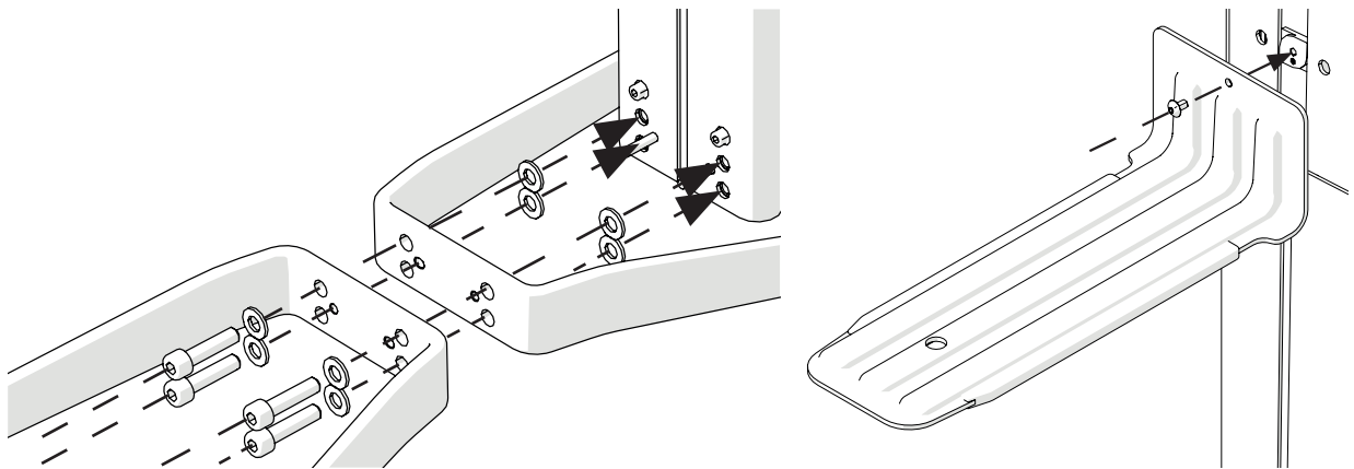
Fig. 3 Assembly steps
