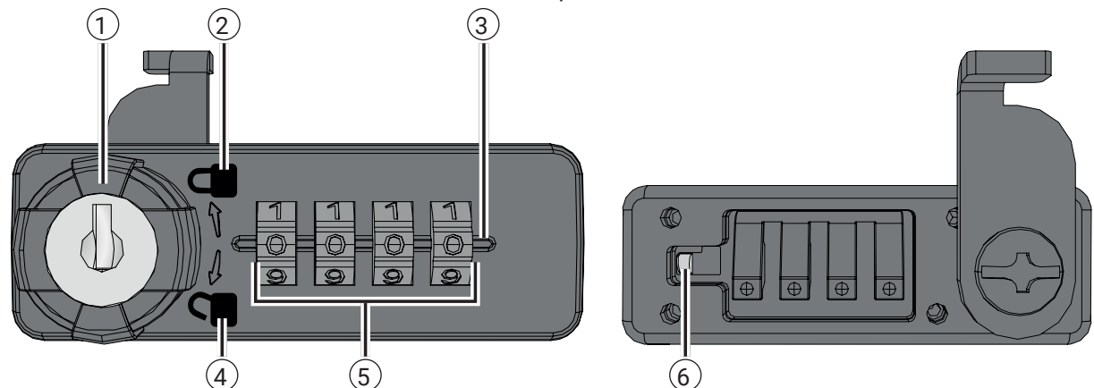
Fig. 4 Lock on the front of the SIGEL office boxes
