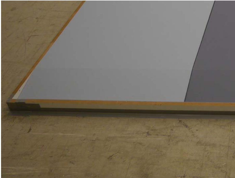
Figure B.3. Circumferential enclosing frame with sealing between frame and floor of the reverberation room.
